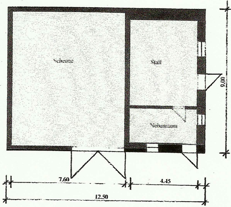
Grundriß Scheune
